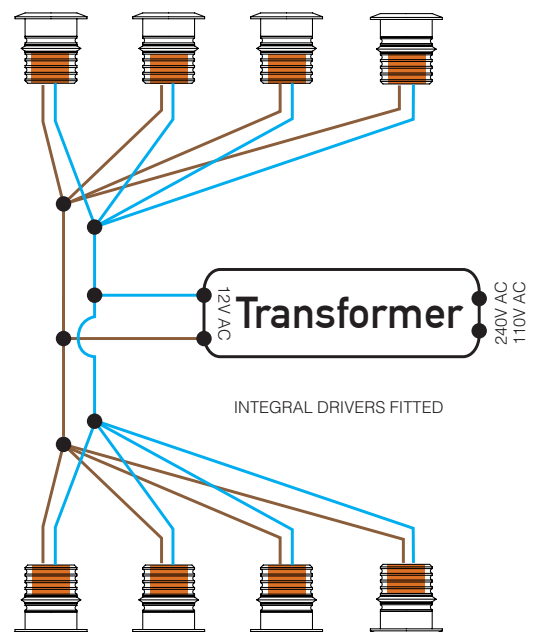
Parallel wiring schematic (if integral driver fitted)
