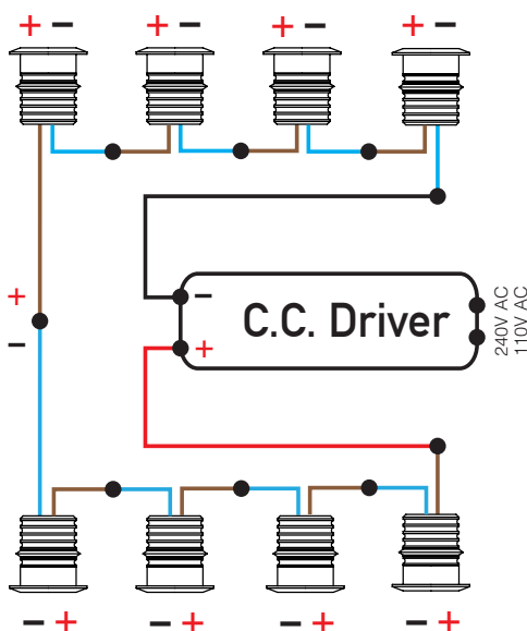
Series wiring schematic (no integral driver fitted)
