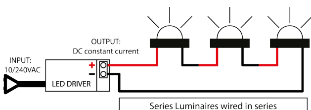
Series wiring schematic (No integral driver)
