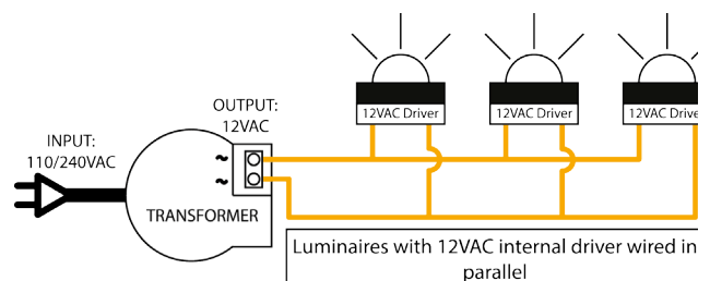
Parallel wiring schematic (Integral driver)
